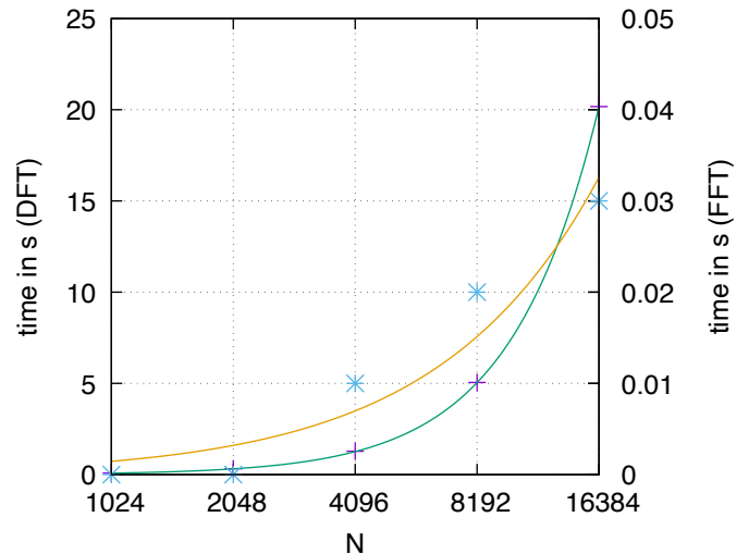
runtime of the DFT and FFT routine
